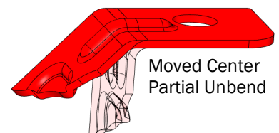
Springback Overbend
